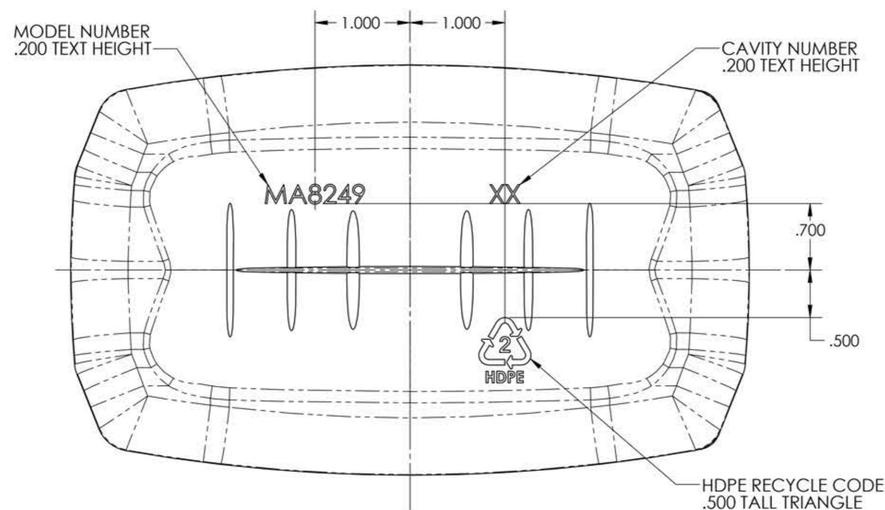
ALL BOTTOM ENGRAVING RAISED .010-.012
