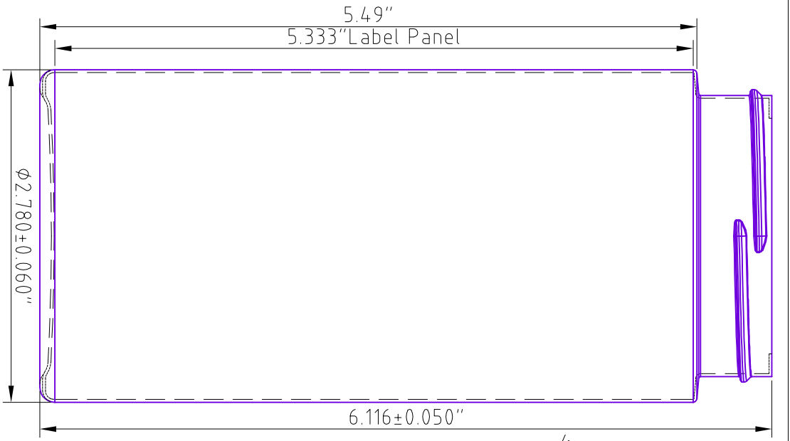
FRONT VIEW
