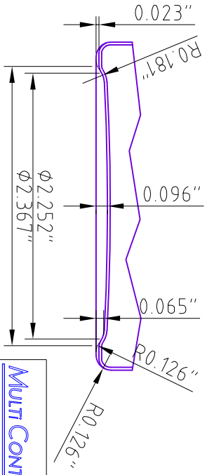
BOTTOM DETAIL, SECTION VIEW
